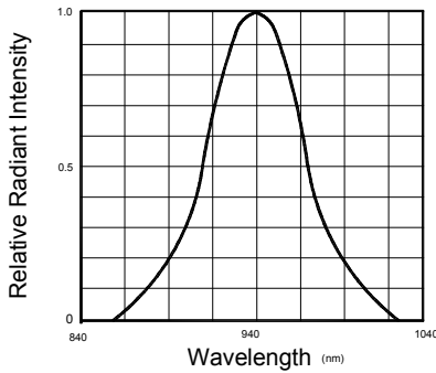
Fig.1 Spectral Distribution
