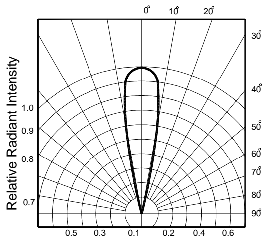
Fig.6 Radiation Diagram
