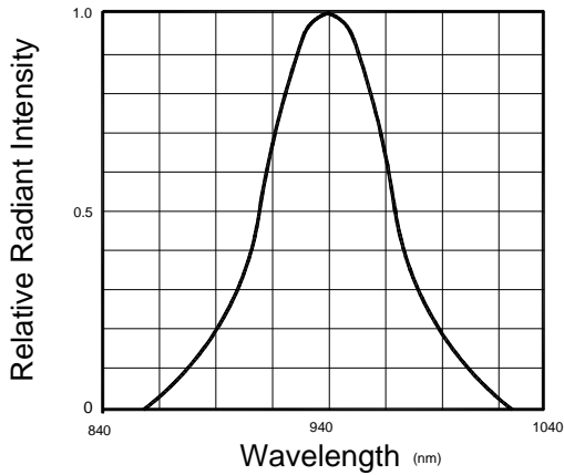
Fig.1 Spectral Distribution
